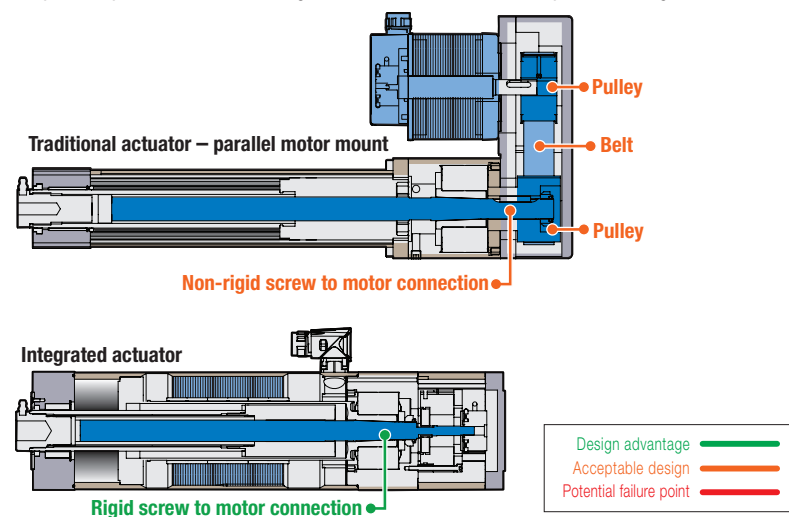
Figure 10: Integrated actuator's rigid motor connection provides superior positional accuracy and bi-directional repeatability
