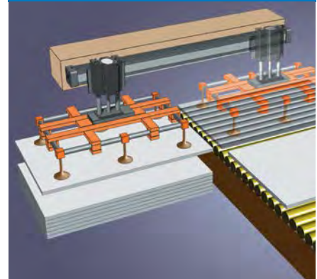
Vacuumized sheet transfer application.
