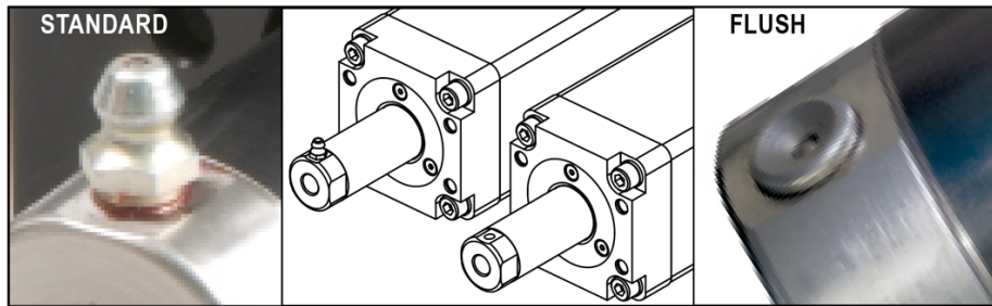
Figure 7.1: A standard or a flush style grease zerk allow periodic relubrication for the GSWA33, 04, 44 & 55 actuator. This can often be done without removing the actuator from its installation.
