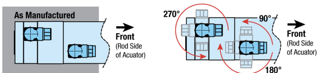
Figure 5.2: Connector rotation. Note that the Tolomatic standard connectors may be rotated from -90° to +180° allowing for cables to connect toward the front (rod end, as manufactured), to either side, both sides, or back of actuator.
