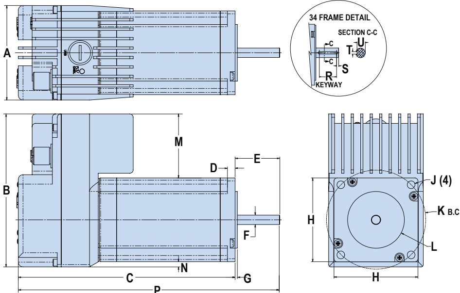
Figure 2-1: ACSI Motor/Drive/Controller Dimensions
