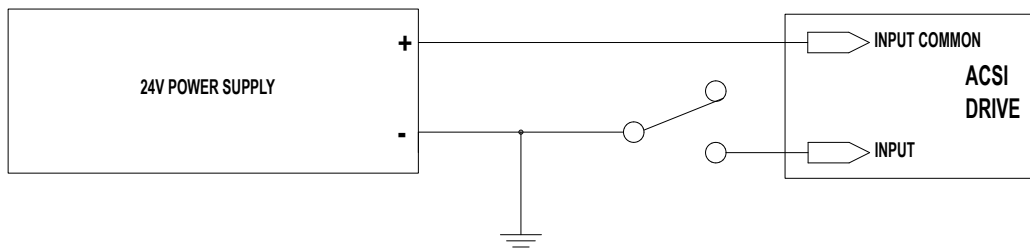
Figure 6-4: Input Sink (switched) Connection
