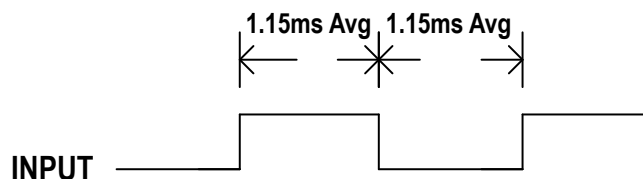
Figure 7-1: Input Requirement
