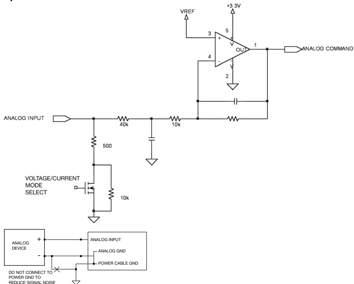
Figure 6-9: Analog Input Equivalent Circuit
