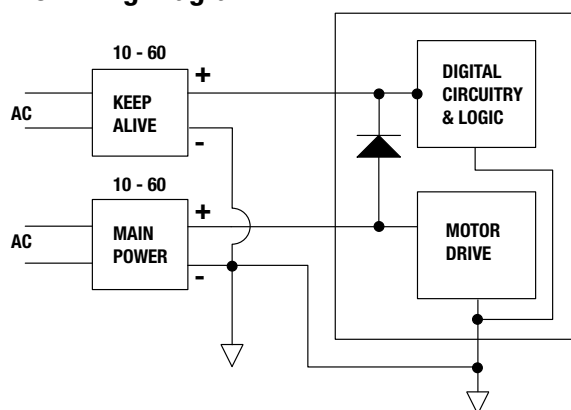
Figure 6-13: Keep Alive wiring diagram
