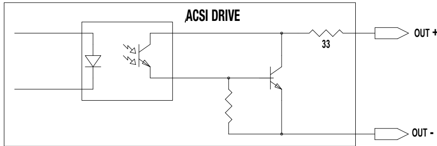
Figure 6-6: Output Circuit
