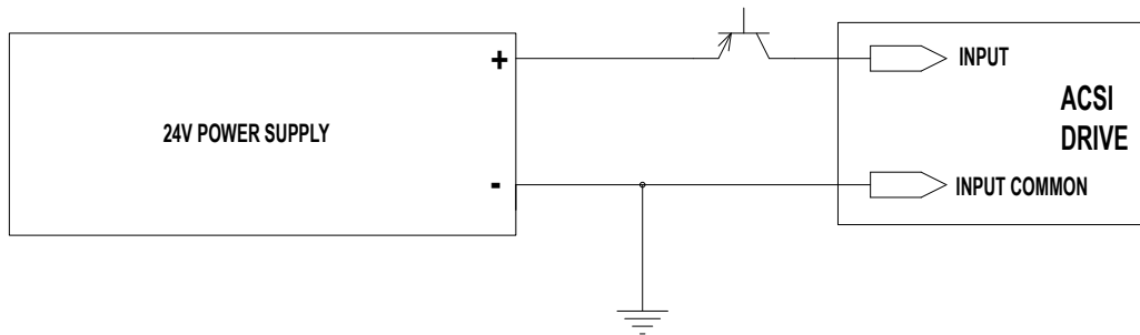
Figure 6-3: Input Source (PNP) Connection
