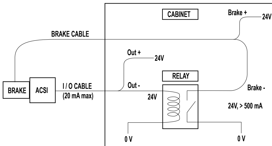
Figure 6-11: Brake output wiring diagram
