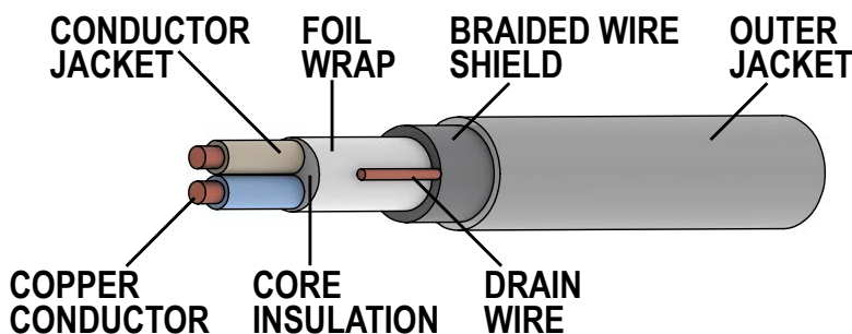
Figure 5-2: Shielded wire diagram
