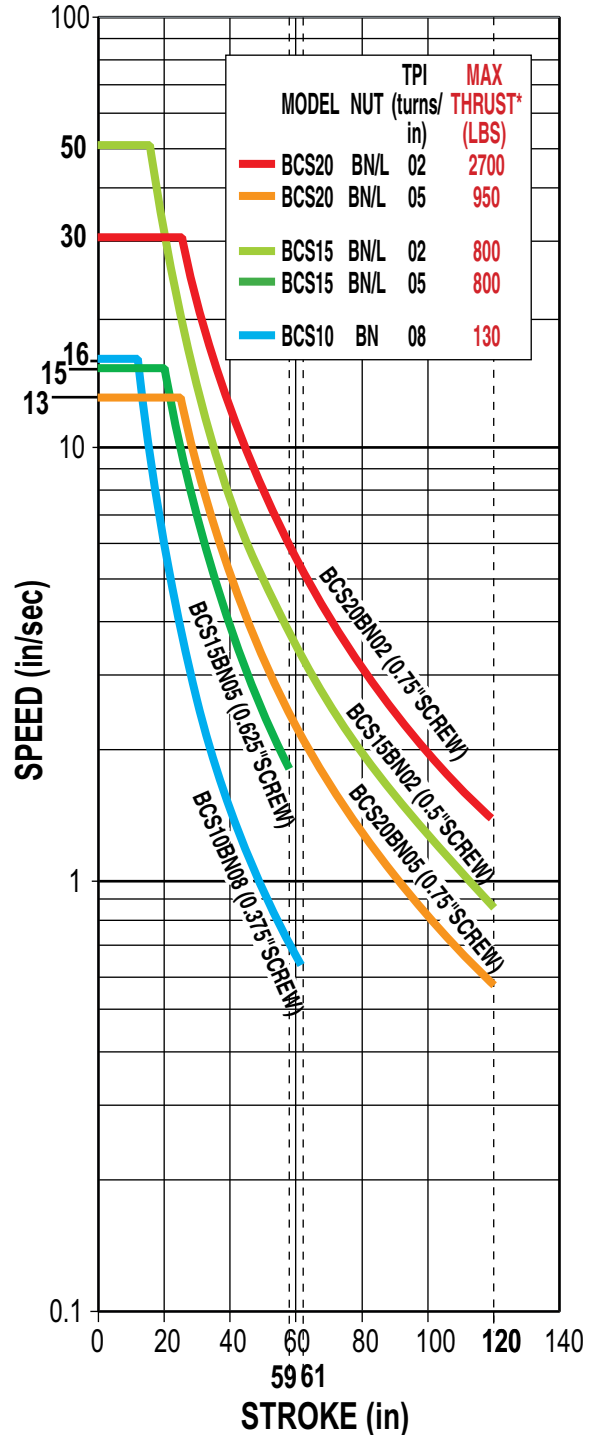
CRITICAL SPEED WITH US CONVENTIONAL BALL SCREW
