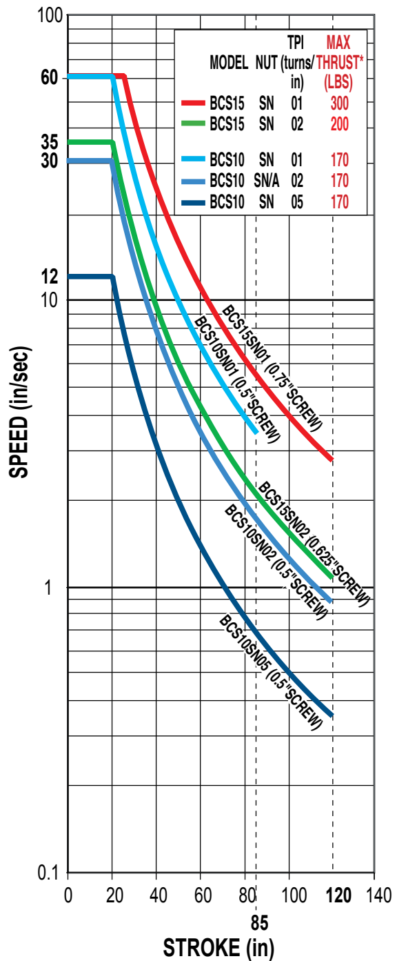
CRITICAL SPEED WITH US CONVENTIONAL ACME SCREW
