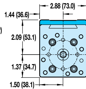
MOTOR MOUNTING
