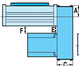
REVERSE-PARALLEL BOTTOM (RPB)
