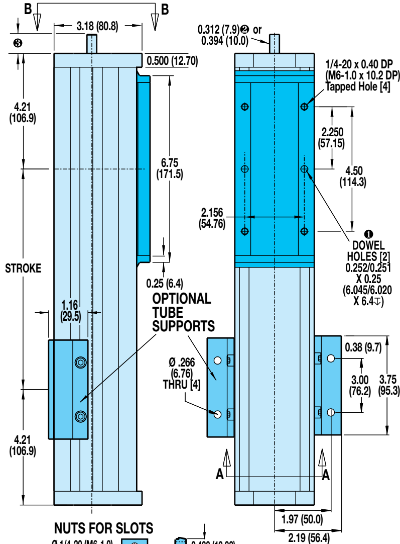
OPTIONAL TUBE SUPPORTS
