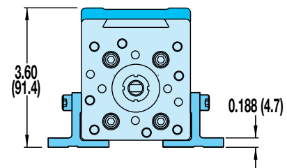
OPTIONAL MOUNTING PLATES
