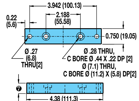
OPTIONAL MOUNTING PLATES
