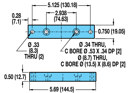
OPTIONAL MOUNTING PLATES
