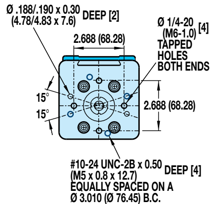
MOTOR MOUNTING
