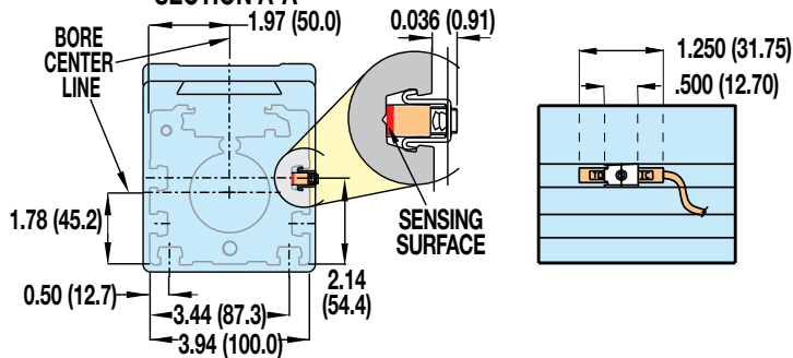
OPTIONAL SWITCH MOUNTING SECTION A-A
