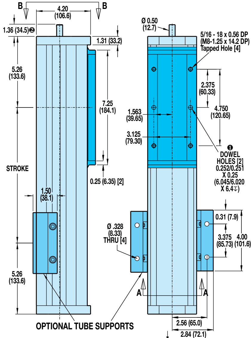
OPTIONAL TUBE SUPPORTS
