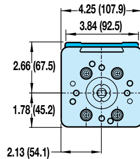
VIEW B-B
