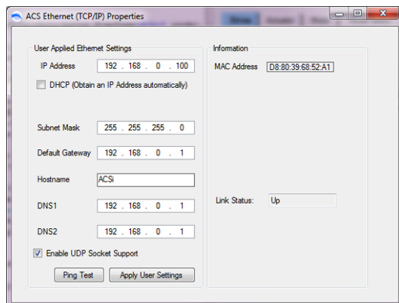
Figure 4-2: Ready to Manually Enter the IP Address for ACSi -MBTCP
