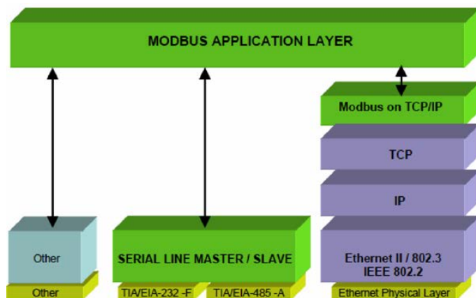
Figure 1-1: Modbus Application Layer
