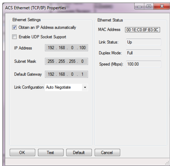
Figure 4-6: Obtaining an IP Address Automatically
