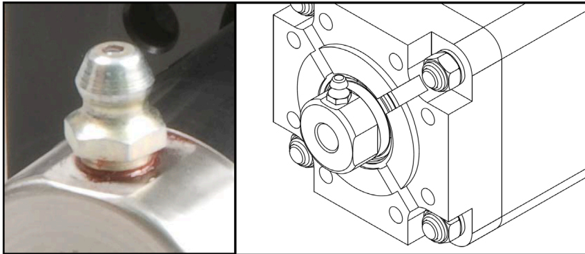
Figure 7.1: A standard grease zerk allows periodic relubrication for ServoWeld actuators. This can typically be performed in 5 minutes without removing the actuator from its installation.
