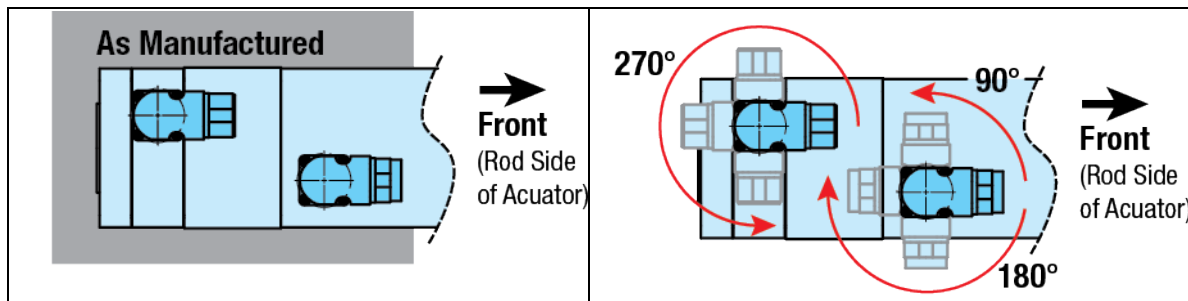
Figure 5.2: Connector rotation. Note that the Tolomatic standard connectors may be rotated from -90^\circ to +180^\circ allowing for cables to connect toward the front (rod end, as manufactured), to either side, both sides, or back of actuator.
