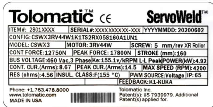
Figure 2.2: ServoWeld CSWX actuator identification label for actuators made in the USA.
