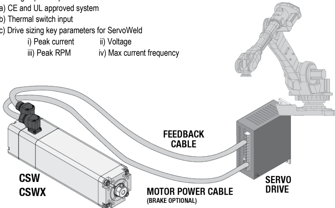
Figure 4.1: Typical connections for a single-axis system with a ServoWeld™ actuator with optional brake to a RSW servo system drive
