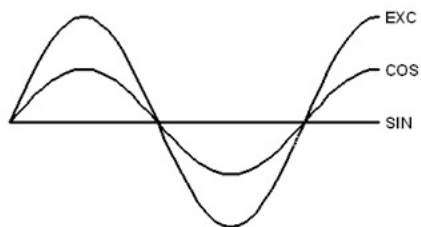
Figure 5.5: Motor rotational position at 0
