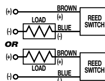
REED SWITCH FORM A LABEL COLOR: RED 10VA MAX. 200 Vdc 500mA Max. Current
