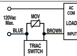
TRIAC SWITCH
