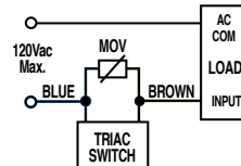
TRIAC SWITCH LABEL COLOR: BLUE Max. 1Amp. Cont. Current @ 86°F Max. .5Amp. Cont. Current @ 140°F Peak surge current 10 Amp.
