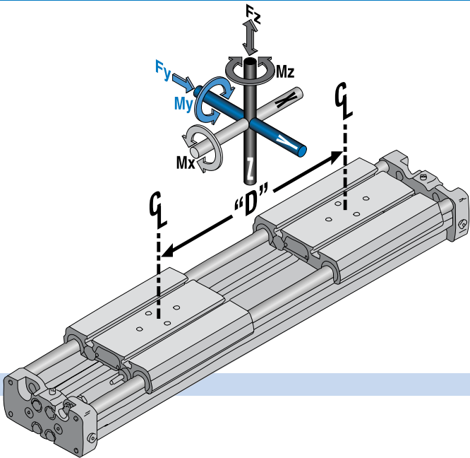
LS10 AUXILIARY CARRIER LOAD vs DISTANCE “D” (Meters)
